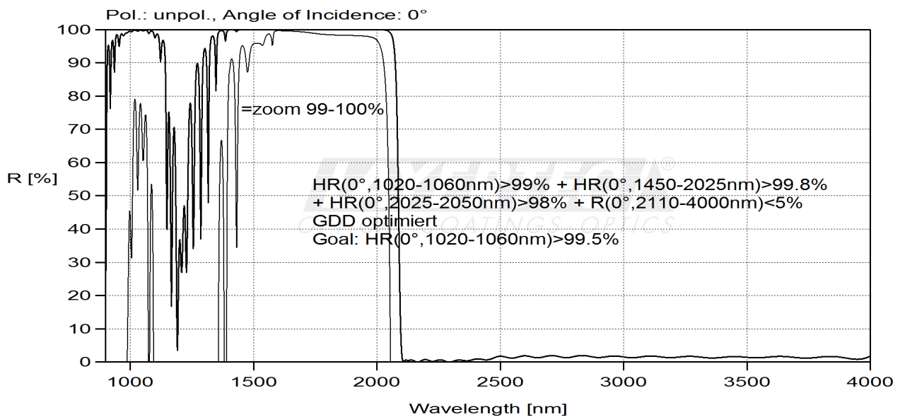
fig. 1 reflection, 0^\circ
